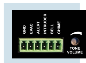
5 Tone Generator
