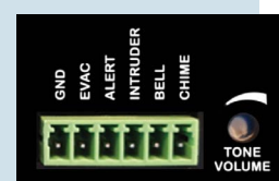
5 Tone Generator
